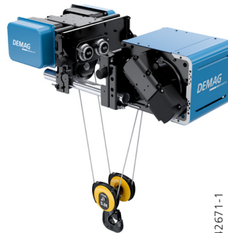
EK-DVR: Low Headroom Monorail Hoist
